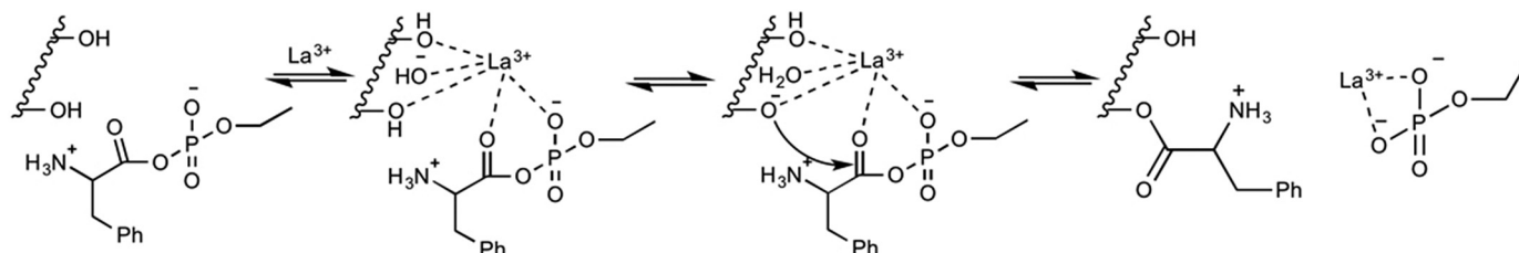
Scheme 1. Lanthanum-promoted monoacylation of the diol in a nucleotide via a chelate formation.
