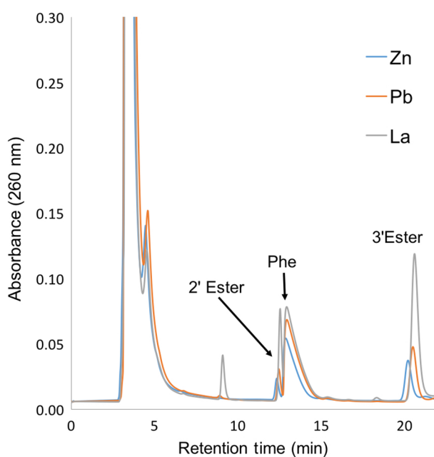
Fig. 1. Amionacylation reaction with adenosine monophosphate (AMP) and phenylalanyl ethyl phosphate (PheEtP) catalyzed by \text{La}^{3+} , \text{Pb}^{2+} , and \text{Zn}^{2+} .
