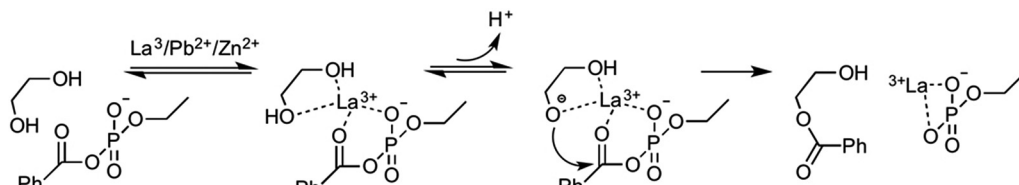
Scheme 2. Lanthanum/lead/zinc-mediated monobenzoylation of ethylene glycol.
