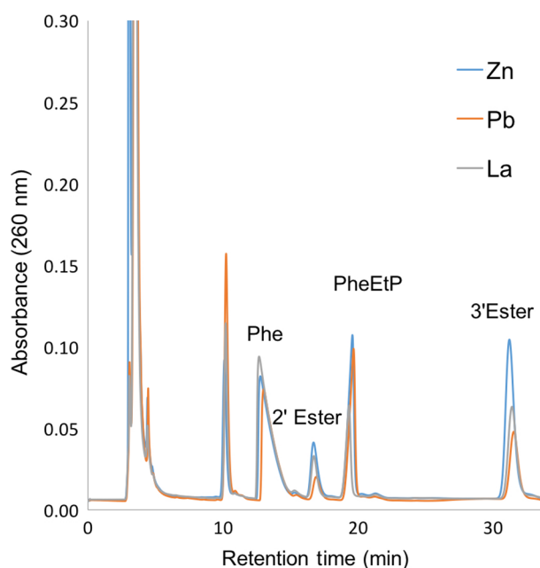
Fig. 2. Aminoacylation reaction with 5'-phospho-2'-deoxyribocytidylriboadenosine (dCA) and phenylalanyl ethyl phosphate (PheEtP) catalyzed by \text{La}^{3+} , \text{Pb}^{2+} , and \text{Zn}^{2+} .
